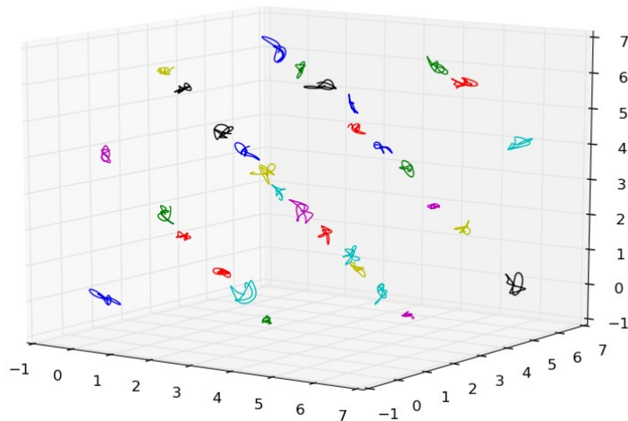
Al 111 plane
