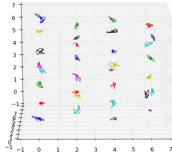
Al(100) plane
